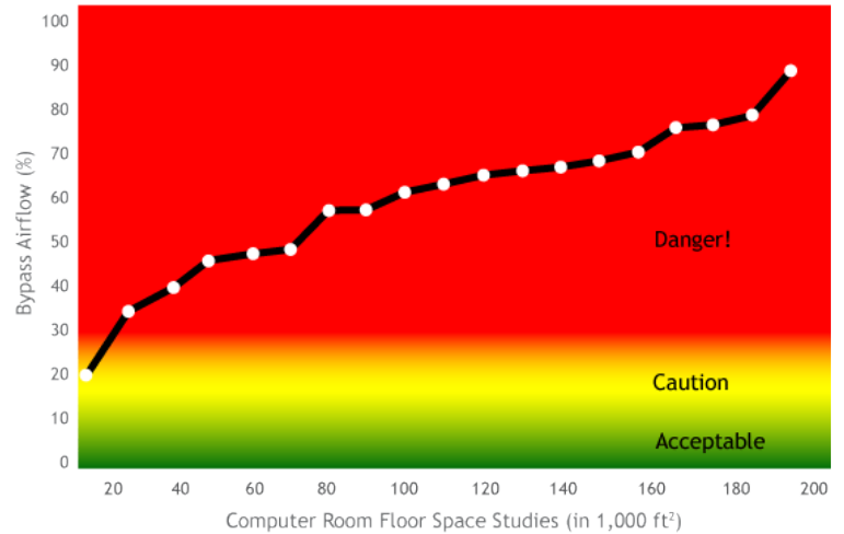
Bypass Airflow in Nineteen Computer Rooms Totaling 204,400 ft 2 (18,952 m 2 )
